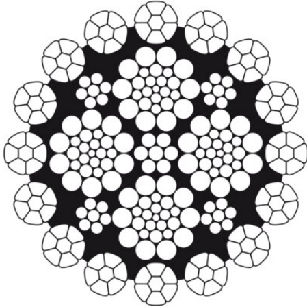
Tower crane
